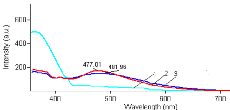
Figure 3. PL spectrum of the pure polystyrene and PS+Si nanocomposite: 1) Pure polystyrene; 2) PS+1%Si; 3) PS+3%Si
